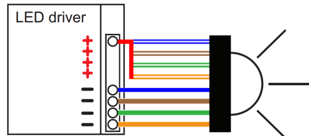
1 Fixture per driver - Common positive format
